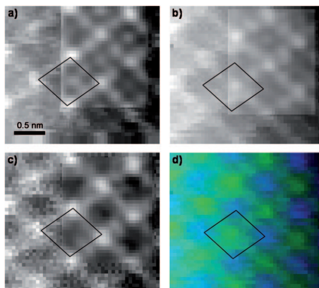
Figure 2. Atomically resolved chemical information on an individual nanocrystal. a) HAADF signal acquired simultaneously with the EELS signal, b) \text{Zr-M}_{2,3} , and c) \text{Ce-M}_{4,5} atomic-resolution chemical maps obtained on a (nominally) \text{Ce}_2\text{Zr}_2\text{O}_8 nanocrystal. Inset images correspond to the experimental data after applying a low-pass filter. d) Experimental Zr (green) and Ce (blue) composite map.
